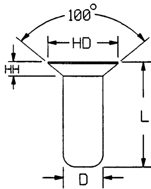
Countersunk Head
