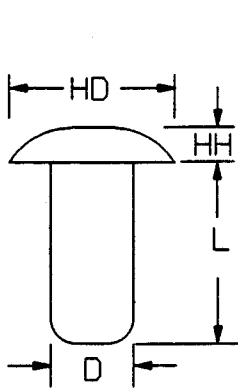
Universal Head
