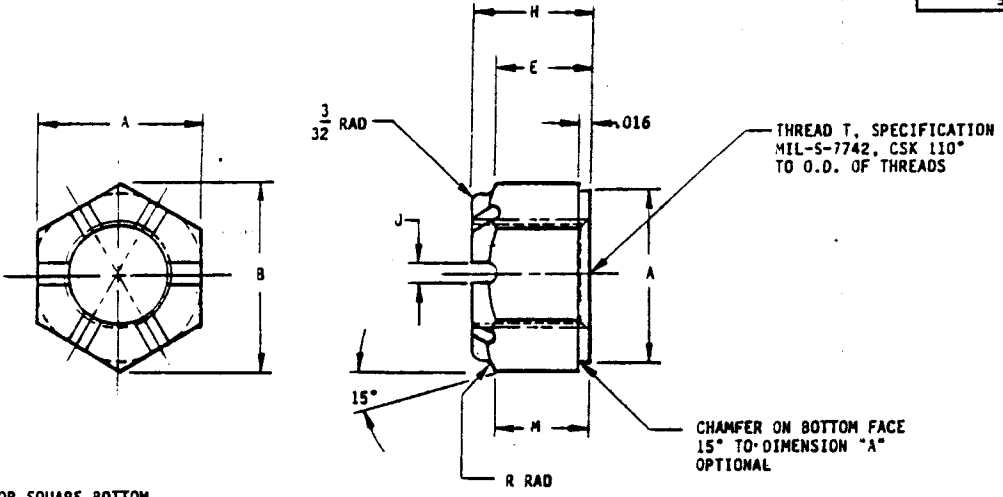
ROUND OR SQUARE BOTTOM CASTELLATION OPTIONAL
